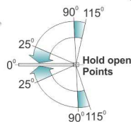
TCH-9400 BM Double Spring Floor Hinge
