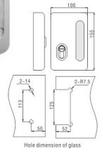
TCH-8508 Sliding Door Lock with Strike Plate
