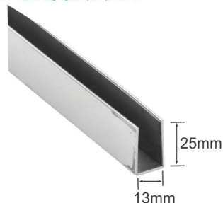
TCH-8467 (CP) 'U' Channel (For Fixed Glass) Available in 3 Mtr. Thickness: 1.5mm Material : SS 304
