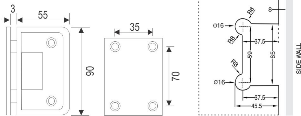
Size & Cutout Details for TCH-8425 & TCH-8431 Wall to Glass 90° Off Set Hinge
