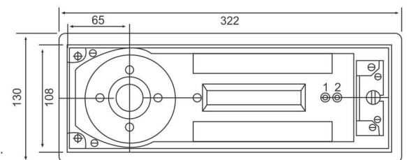
TCH-9400 GD Double Spring Floor Hinge
