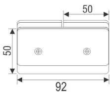
Size & Cutout Details for TCH-8443, TCH-8443 A & TCH-8443 R Glass to Glass 180° Connector
