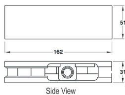
TCH-001 BM Top Patch
