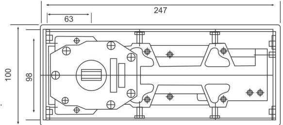
TCH-8400 GD Double Spring Floor Hinge
