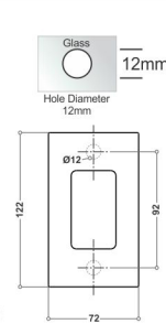
TCH-8507 Sliding Handle (Rectangle)
