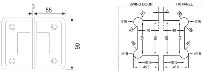
Size & Cutout Details for TCH-8427 & TCH-8433 Glass to Glass 180° Hinge
