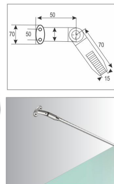
TCH-8518 Wall to Rod Connector
