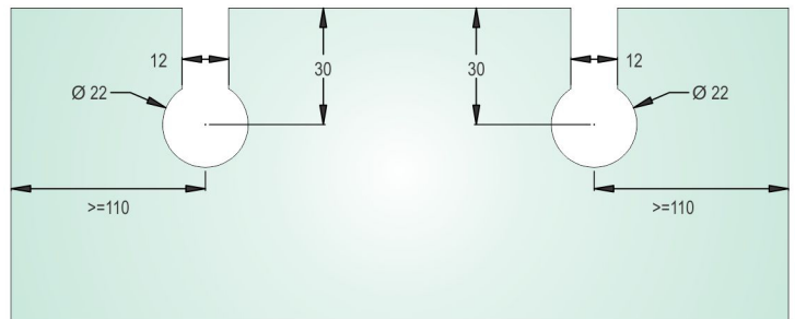
CUTOUT DETAILS OF TCH-8496
