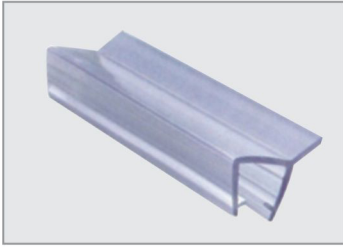
TCH-8445 Wall Seal For : 10-12mm Glass, Size : 2.2mtr.
