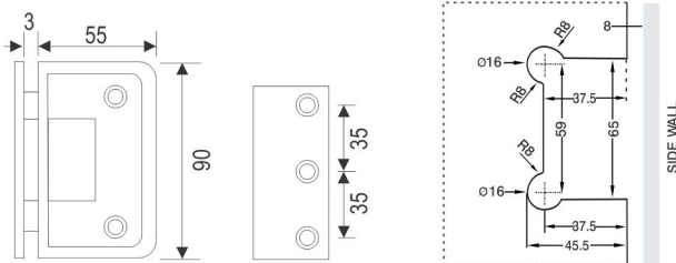
Size & Cutout Details for TCH-8426 & TCH-8432 Wall to Glass 90° Hinge
