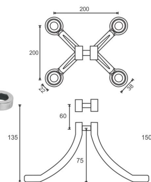
TCH-8838 Four Way Spider (Wall Mounted)
