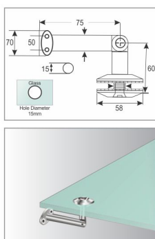
TCH-8516 Wall to Glass Connector
