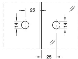
Size & Cutout Details for TCH-8443, TCH-8443 A & TCH-8443 R Glass to Glass 180° Connector
