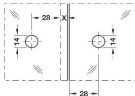
Size & Cutout Details for TCH-8440, TCH-8440 A & TCH-8440 R Glass to Glass 90° Connector
