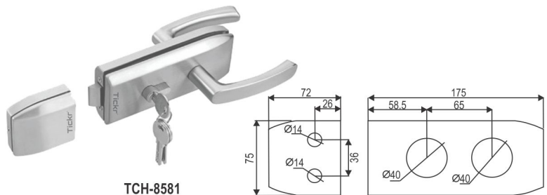
TCH-8581 Single Door lock (Wall to Glass)
