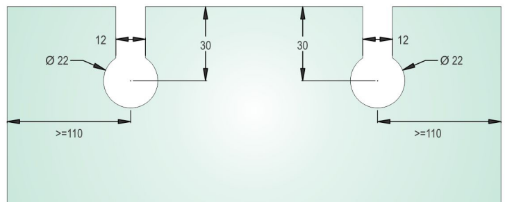
CUTOUT DETAILS OF TCH-8497
