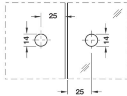
Size & Cutout Details for TCH-8439, TCH-8439 A & TCH-8439 R Glass to Glass 135° Connector
