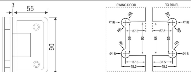
Size & Cutout Details for TCH-8429 & TCH-8436 Glass to Glass 90° Hinge
