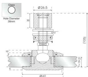
TCH-8537 Articulated Routel (Flat Head)
