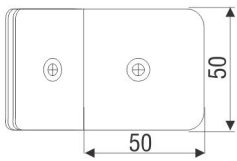
Size & Cutout Details for TCH-8439, TCH-8439 A & TCH-8439 R Glass to Glass 135° Connector
