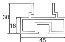
TCH-8829 Top/ Bottom Profile
