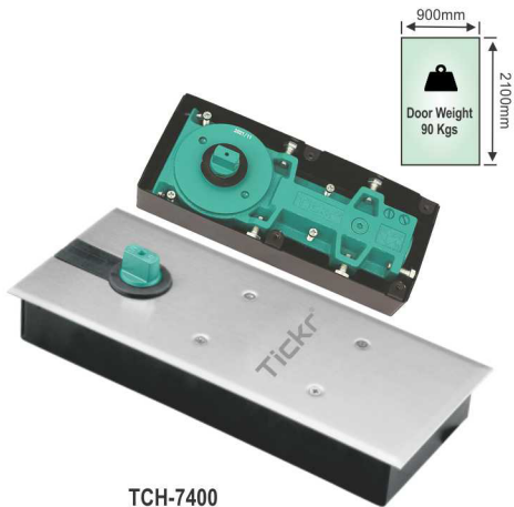
TCH-7400 Single Spring Floor Hinge
