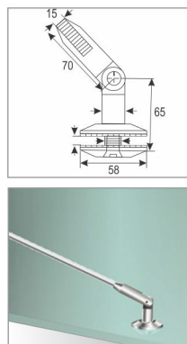
TCH-8517 Rod to Glass Connector
