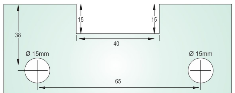
CUTOUT DETAILS OF TCH-8498
