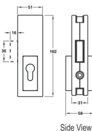
TCH-8407 Corner Patch Lock with Strike Plate
