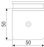
Size & Cutout Details for TCH-8440, TCH-8440 A & TCH-8440 R Glass to Glass 90° Connector
