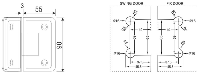
Size & Cutout Details for TCH-84278 & TCH-8435 Glass to Glass 135° Hinge
