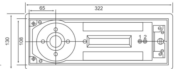
TCH-7400 GD Double Spring Floor Hinge
