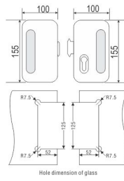
TCH-8506 Sliding Handle (Square)
