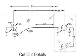
TCH-8406 Over Panel Side Panel Connecting Patch with Pivot (Big L)
