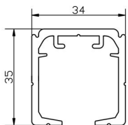
TCH-8828 Sliding Top Track
