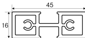
TCH-8833 Divider Profile
